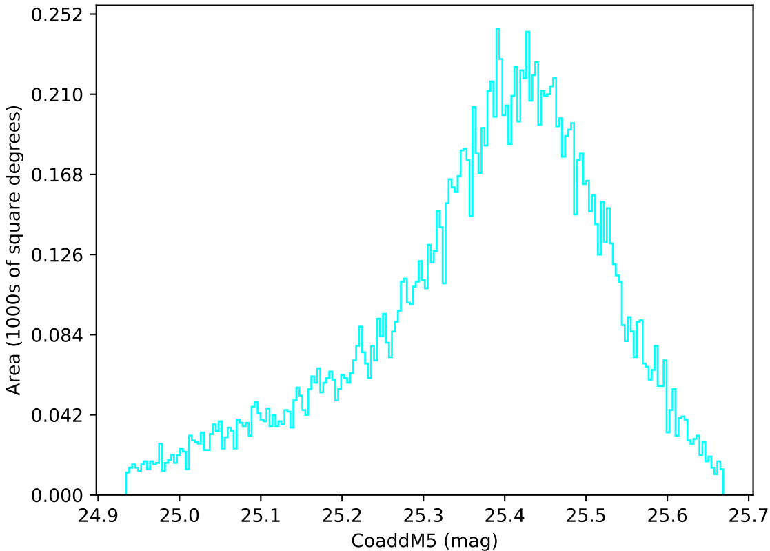
too_elab_r128_d2_gz_v3.4_10yrs WFD u band: CoaddM5
