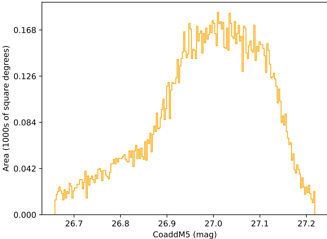
too_elab_r128_d2_gz_v3.4_10yrs WFD r band: CoaddM5
