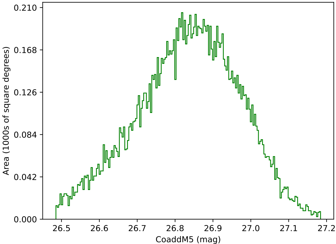
too_elab_r128_d2_gz_v3.4_10yrs WFD g band: CoaddM5
