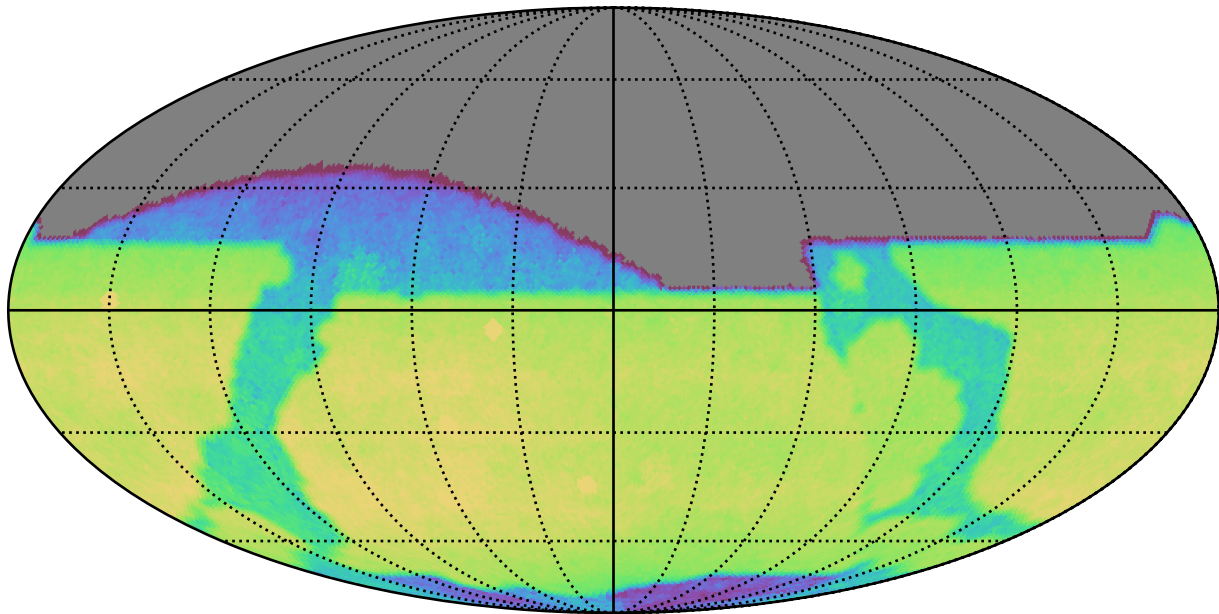
too_elab_r128_d2_gz_v3.4_10yrs All sky z band: CoaddM5
