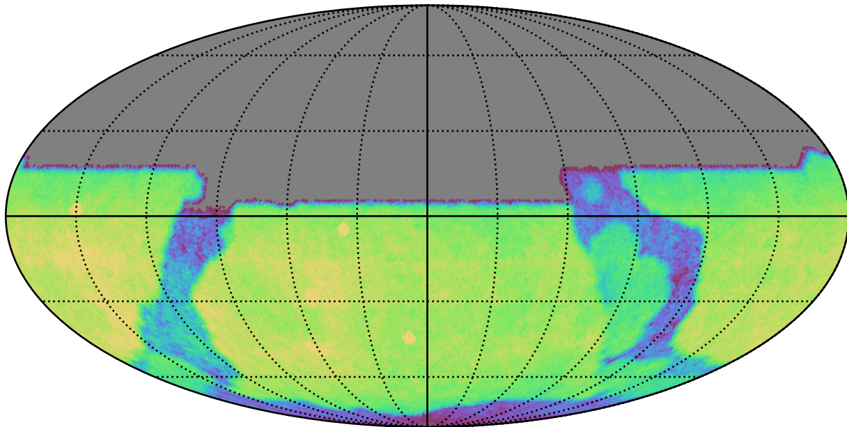
too_elab_r128_d2_gz_v3.4_10yrs All sky u band: CoaddM5
