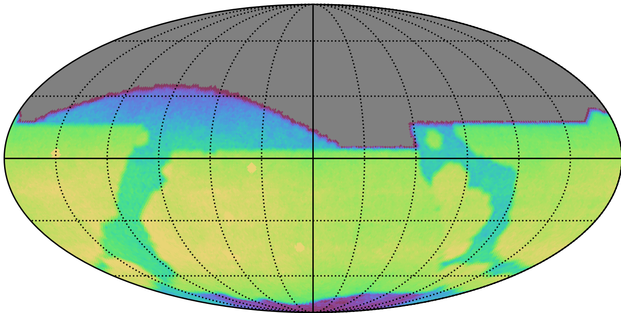
too_elab_r128_d2_gz_v3.4_10yrs All sky r band: CoaddM5
