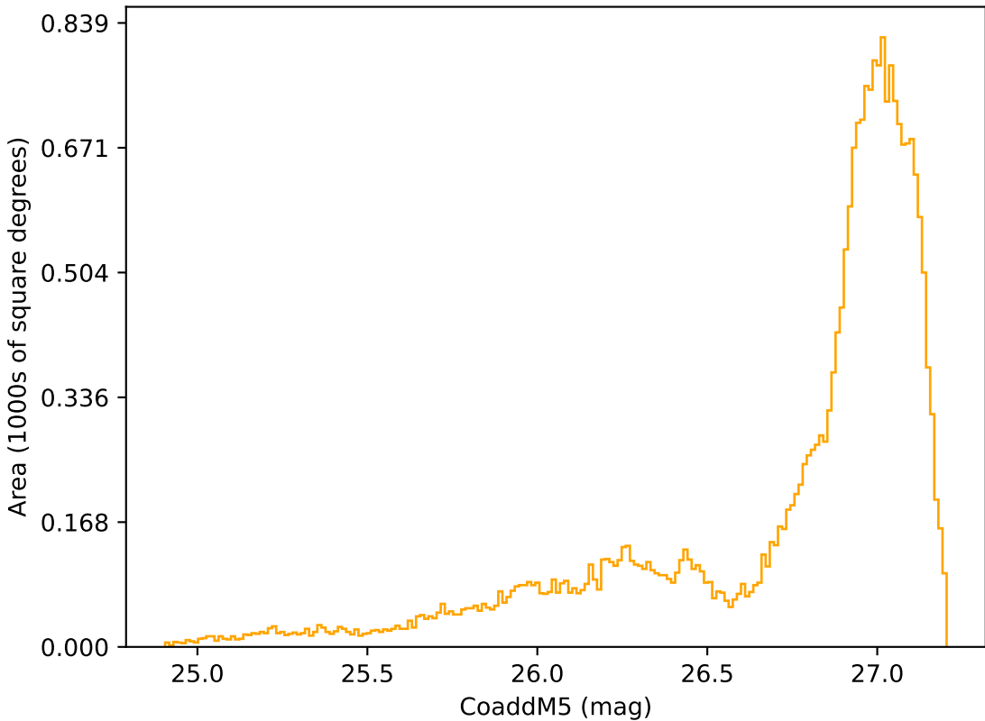
too_elab_r128_d2_gz_v3.4_10yrs All sky r band: CoaddM5
