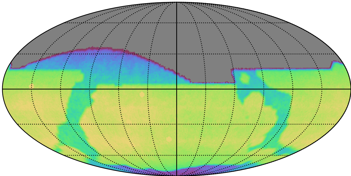
too_elab_r128_d2_gz_v3.4_10yrs All sky i band: CoaddM5
