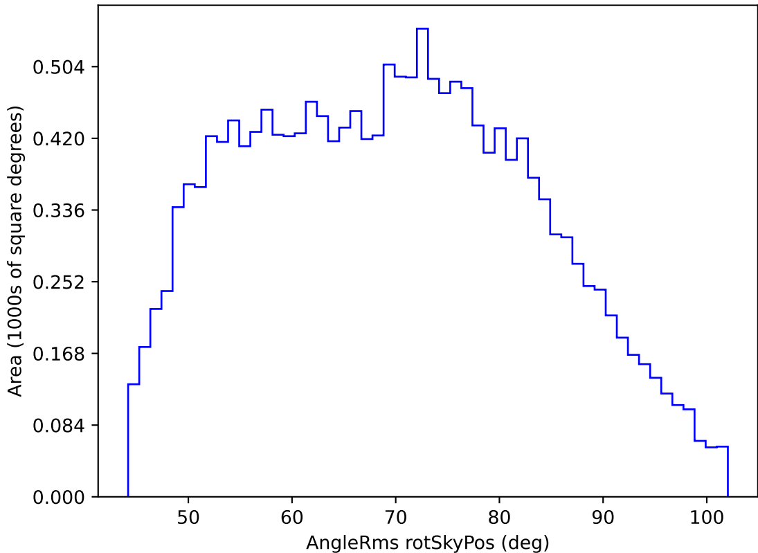
too_elab_r128_d2_gz_v3.4_10yrs WFD g band: AngleRms rotSkyPos
