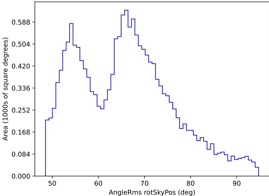
too_elab_r128_d2_gz_v3.4_10yrs WFD all bands: AngleRms rotSkyPos
