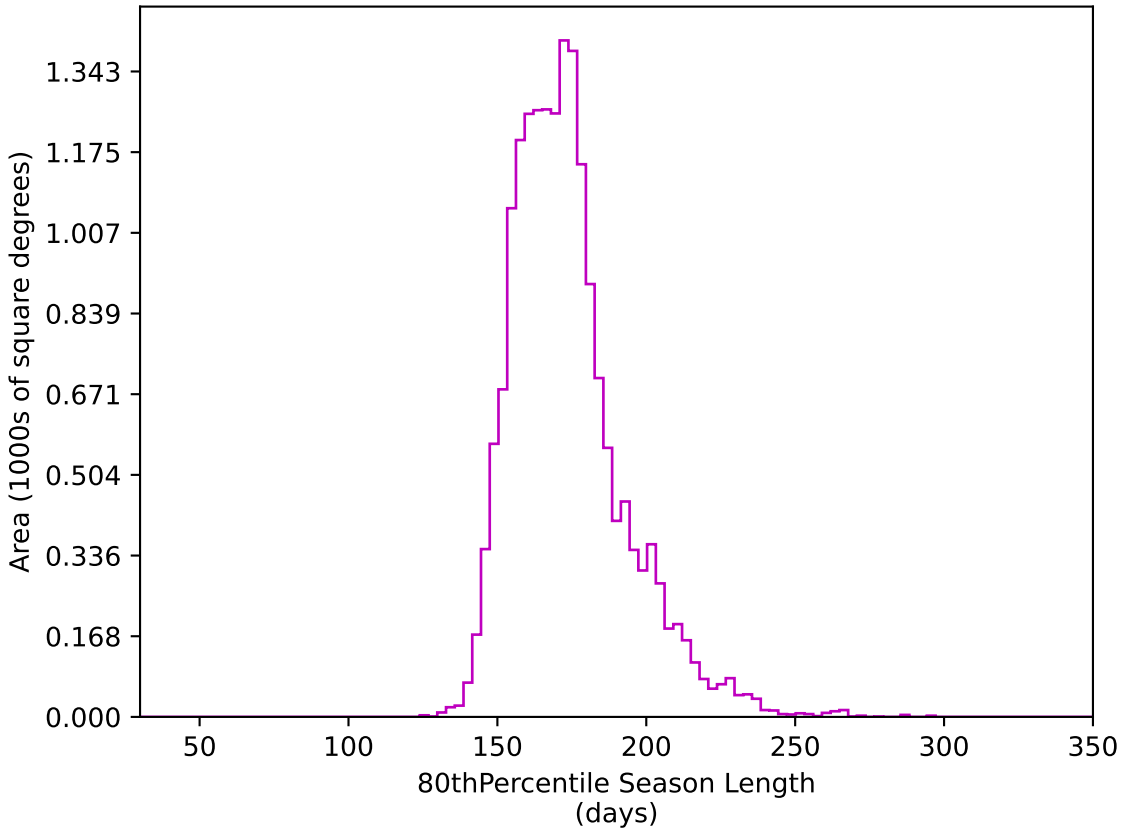
too_elab_r128_d2_gz_v3.4_10yrs WFD z band: 80thPercentile Season Length
