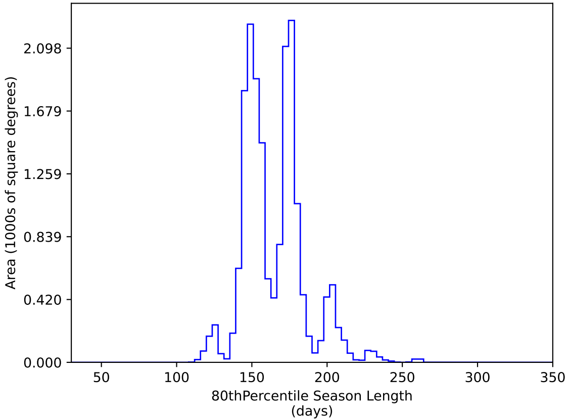
too_elab_r128_d2_gz_v3.4_10yrs WFD y band: 80thPercentile Season Length
