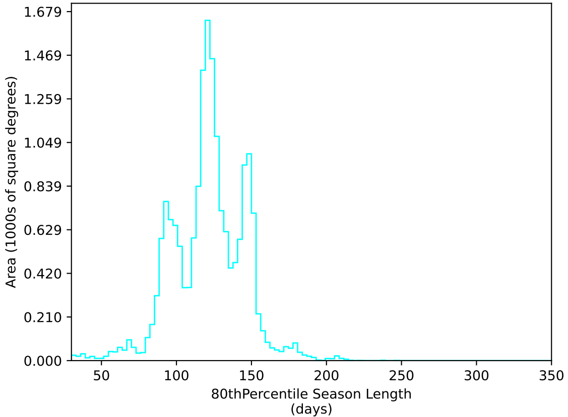
too_elab_r128_d2_gz_v3.4_10yrs WFD u band: 80thPercentile Season Length
