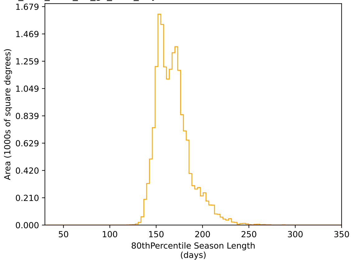
too_elab_r128_d2_gz_v3.4_10yrs WFD r band: 80thPercentile Season Length
