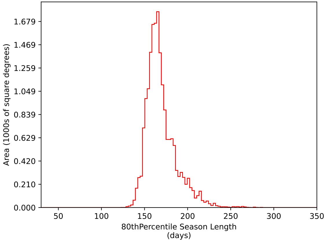
too_elab_r128_d2_gz_v3.4_10yrs WFD i band: 80thPercentile Season Length
