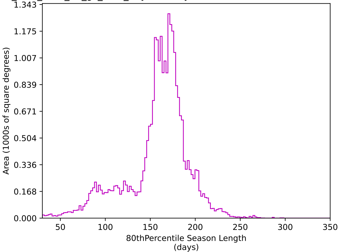
too_elab_r128_d2_gz_v3.4_10yrs All sky z band: 80thPercentile Season Length
