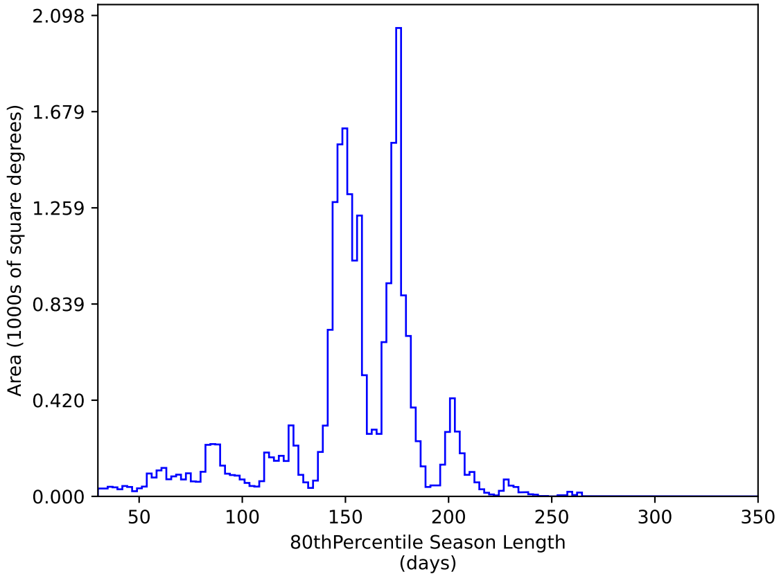
too_elab_r128_d2_gz_v3.4_10yrs All sky y band: 80thPercentile Season Length
