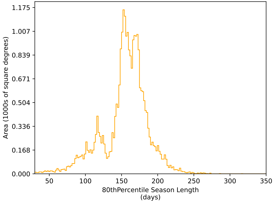
too_elab_r128_d2_gz_v3.4_10yrs All sky r band: 80thPercentile Season Length
