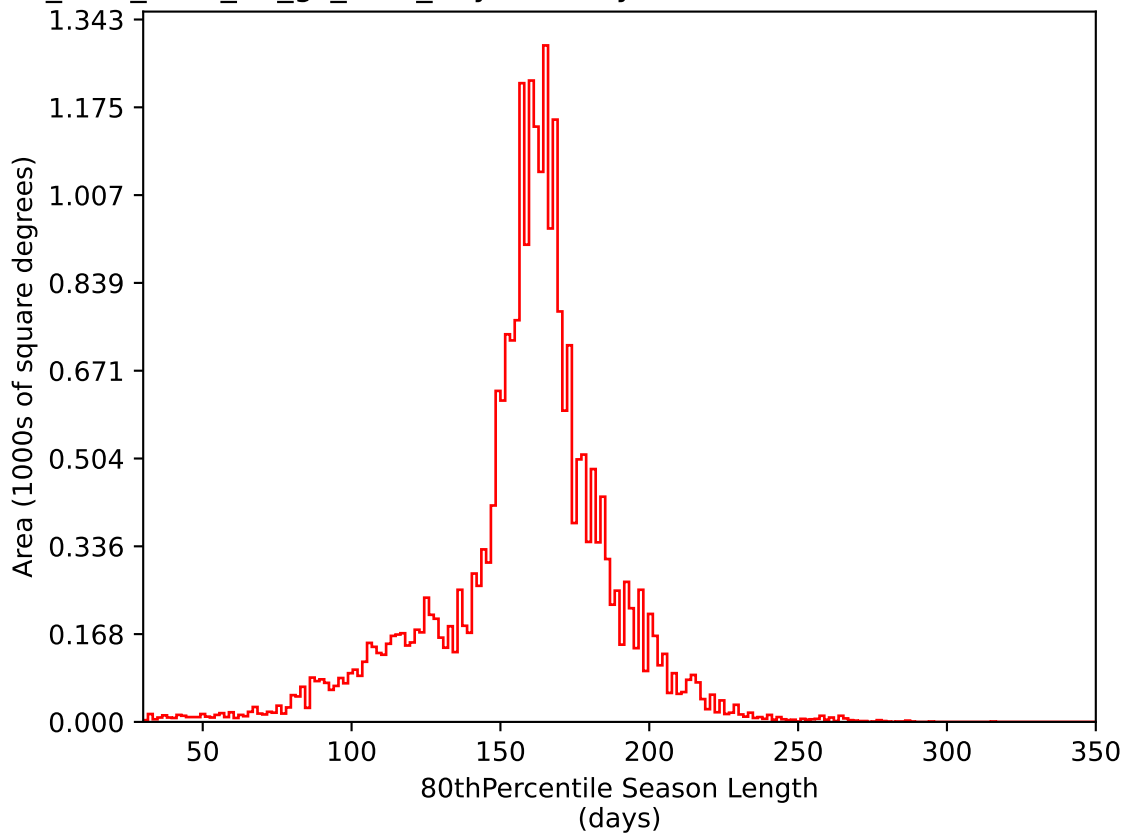
too_elab_r128_d2_gz_v3.4_10yrs All sky i band: 80thPercentile Season Length
