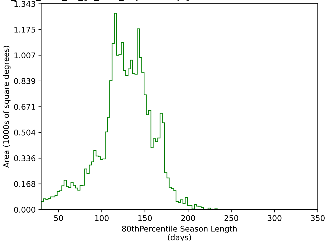
too_elab_r128_d2_gz_v3.4_10yrs All sky g band: 80thPercentile Season Length
