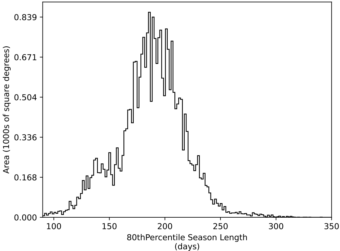
too_elab_r128_d2_gz_v3.4_10yrs All sky all bands: 80thPercentile Season Length
