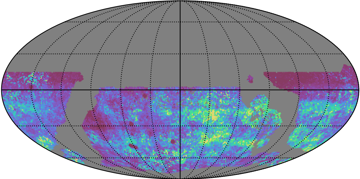
too_elab_r128_d2_gz_v3.4_10yrs WFD zy bands: 75th Percentile Intranight Timespan
