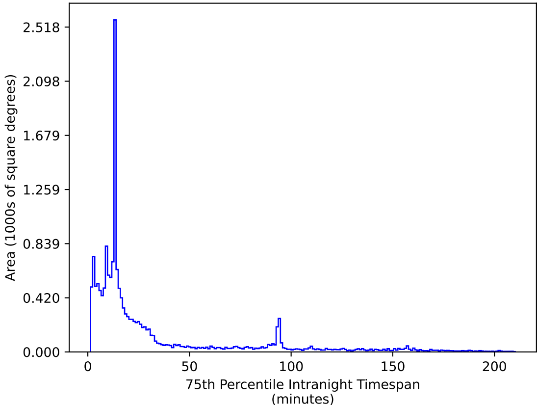
too_elab_r128_d2_gz_v3.4_10yrs WFD z band: 75th Percentile Intranight Timespan
