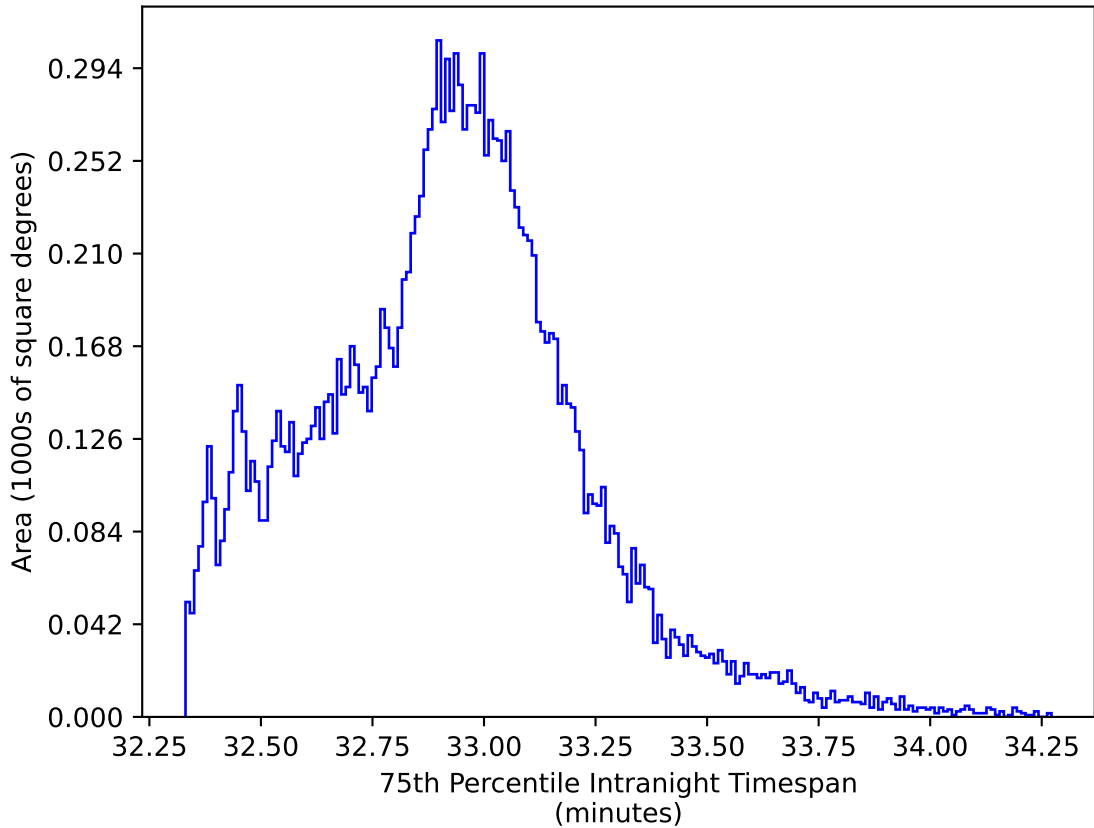
too_elab_r128_d2_gz_v3.4_10yrs WFD y band: 75th Percentile Intranight Timespan
