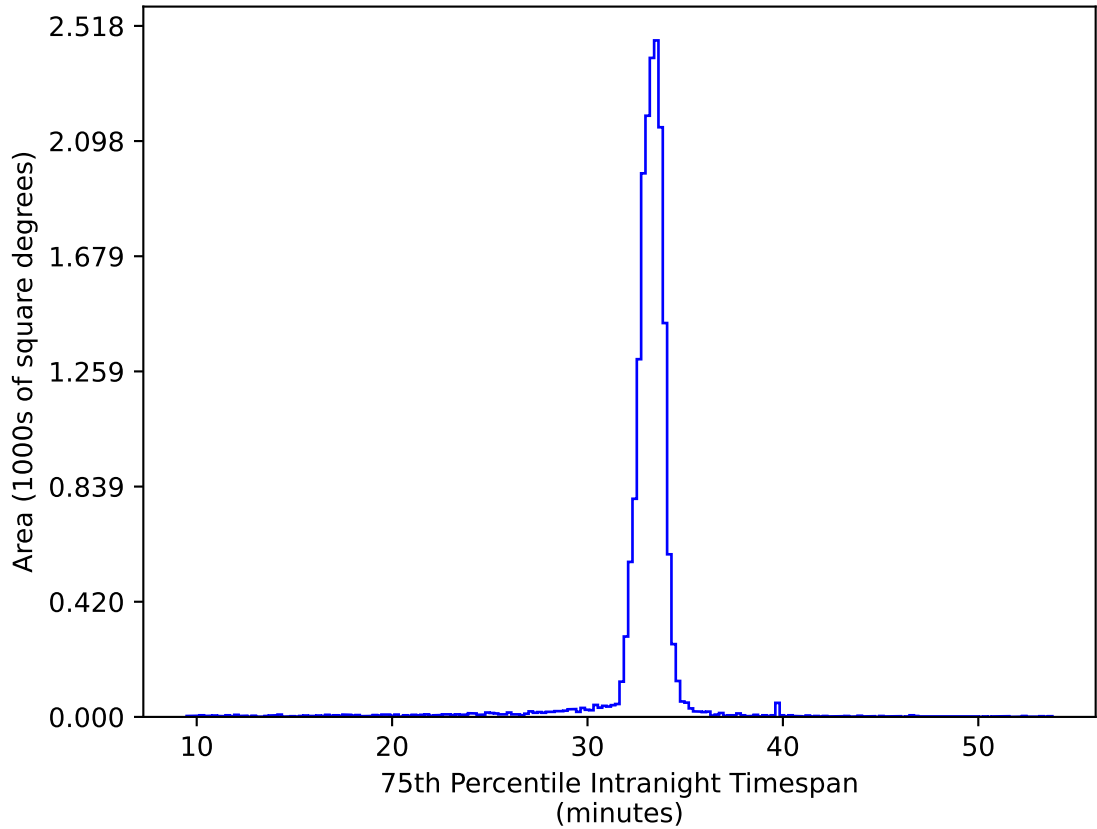
too_elab_r128_d2_gz_v3.4_10yrs WFD ug bands: 75th Percentile Intranight Timespan
