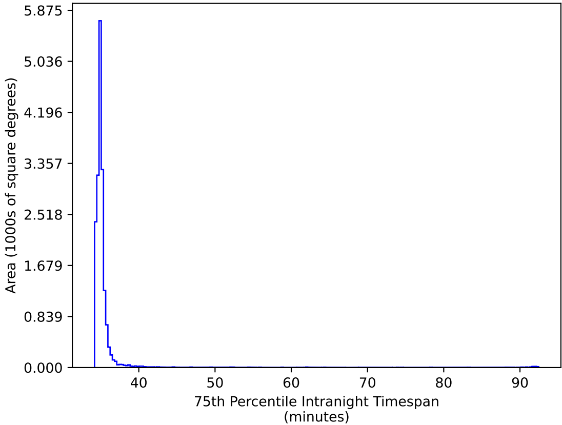
too_elab_r128_d2_gz_v3.4_10yrs WFD ri bands: 75th Percentile Intranight Timespan
