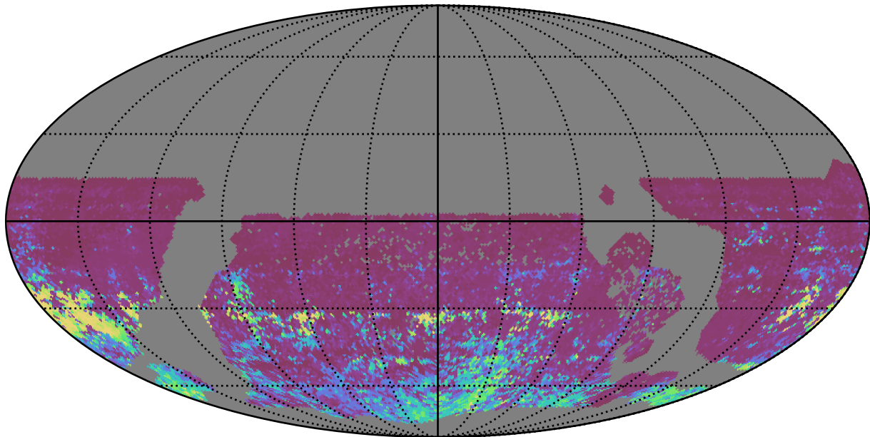
too_elab_r128_d2_gz_v3.4_10yrs WFD r band: 75th Percentile Intranight Timespan
