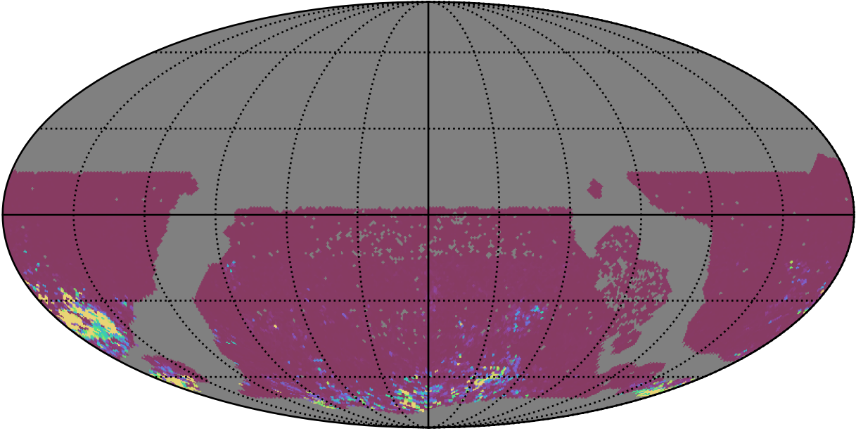
too_elab_r128_d2_gz_v3.4_10yrs WFD gr bands: 75th Percentile Intranight Timespan
