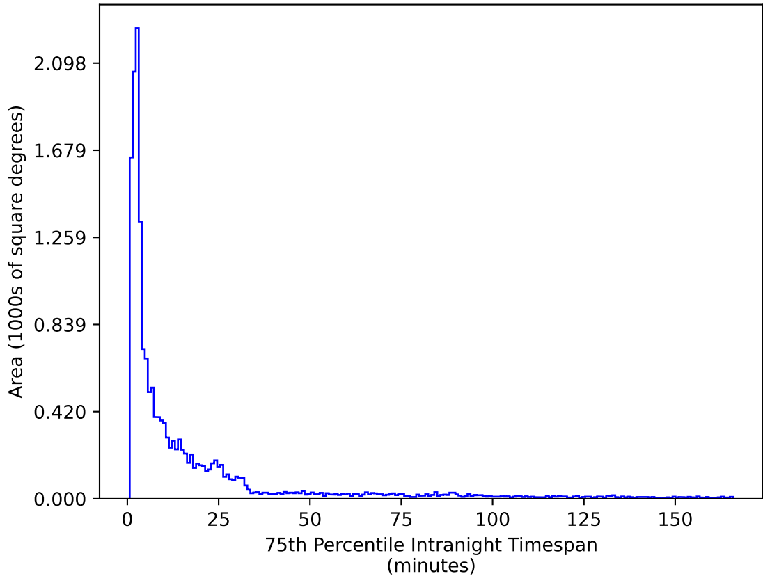
too_elab_r128_d2_gz_v3.4_10yrs WFD g band: 75th Percentile Intranight Timespan
