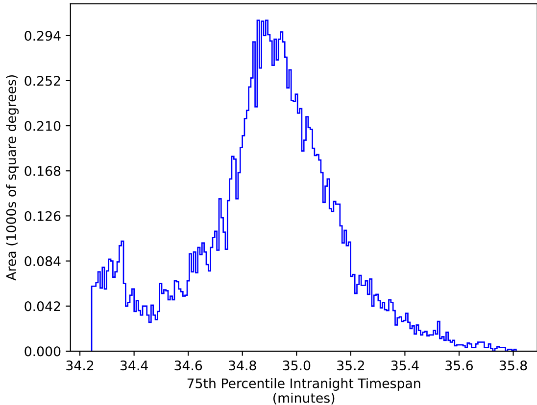
too_elab_r128_d2_gz_v3.4_10yrs WFD: 75th Percentile Intranight Timespan
