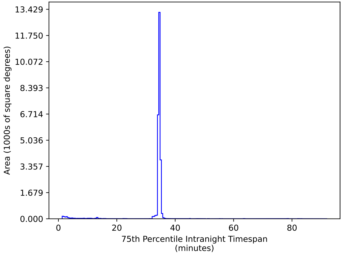
too_elab_r128_d2_gz_v3.4_10yrs All sky zy bands: 75th Percentile Intranight Timespan
