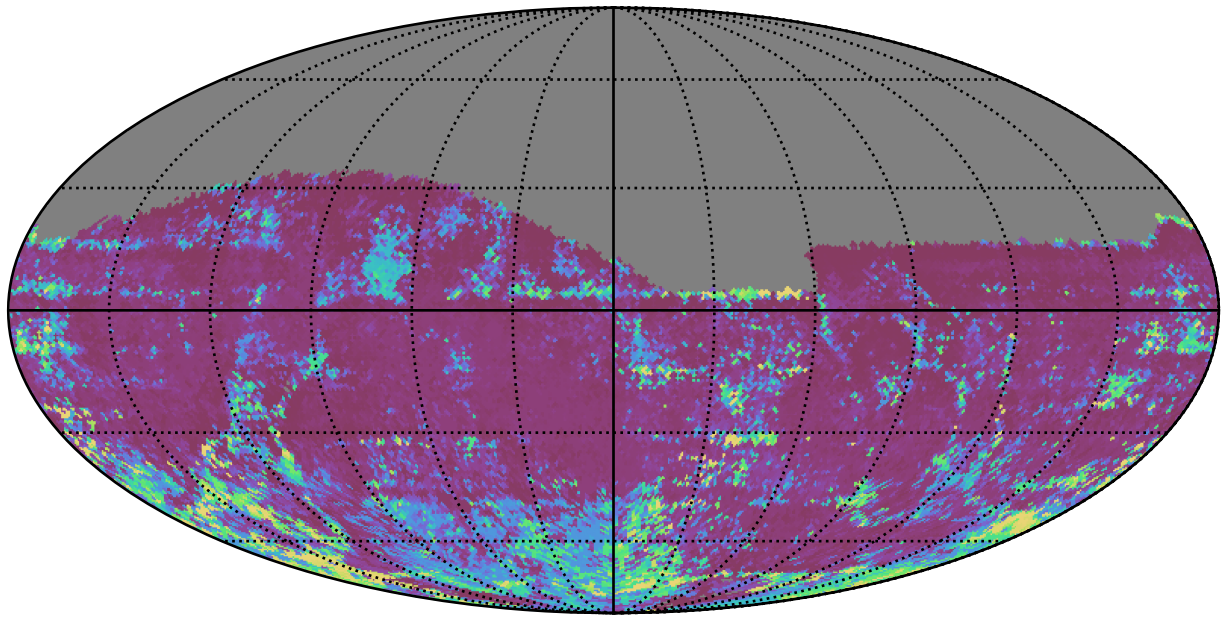
too_elab_r128_d2_gz_v3.4_10yrs All sky z band: 75th Percentile Intranight Timespan
