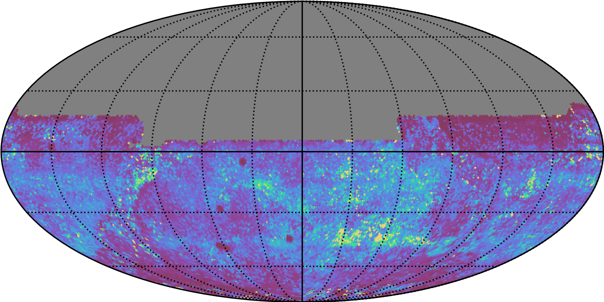
too_elab_r128_d2_gz_v3.4_10yrs All sky y band: 75th Percentile Intranight Timespan
