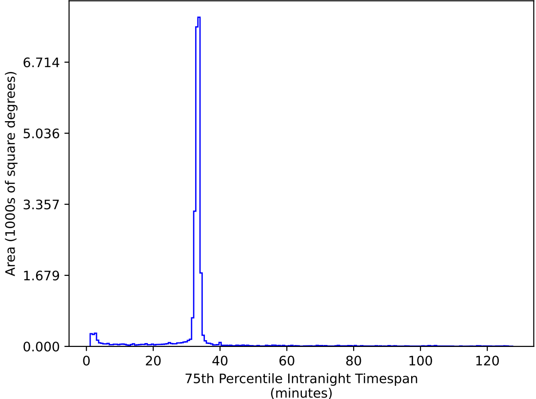
too_elab_r128_d2_gz_v3.4_10yrs All sky ug bands: 75th Percentile Intranight Timespan
