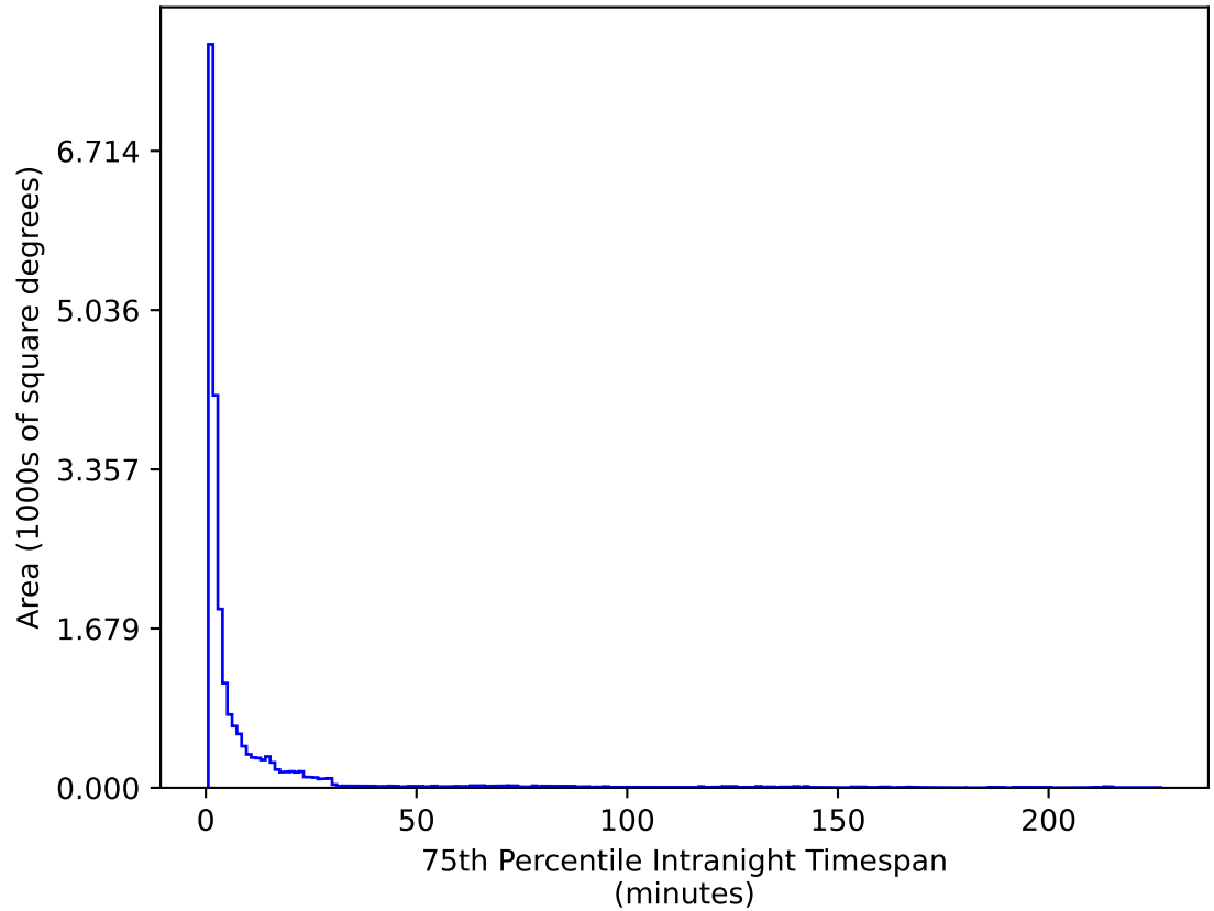
too_elab_r128_d2_gz_v3.4_10yrs All sky u band: 75th Percentile Intranight Timespan
