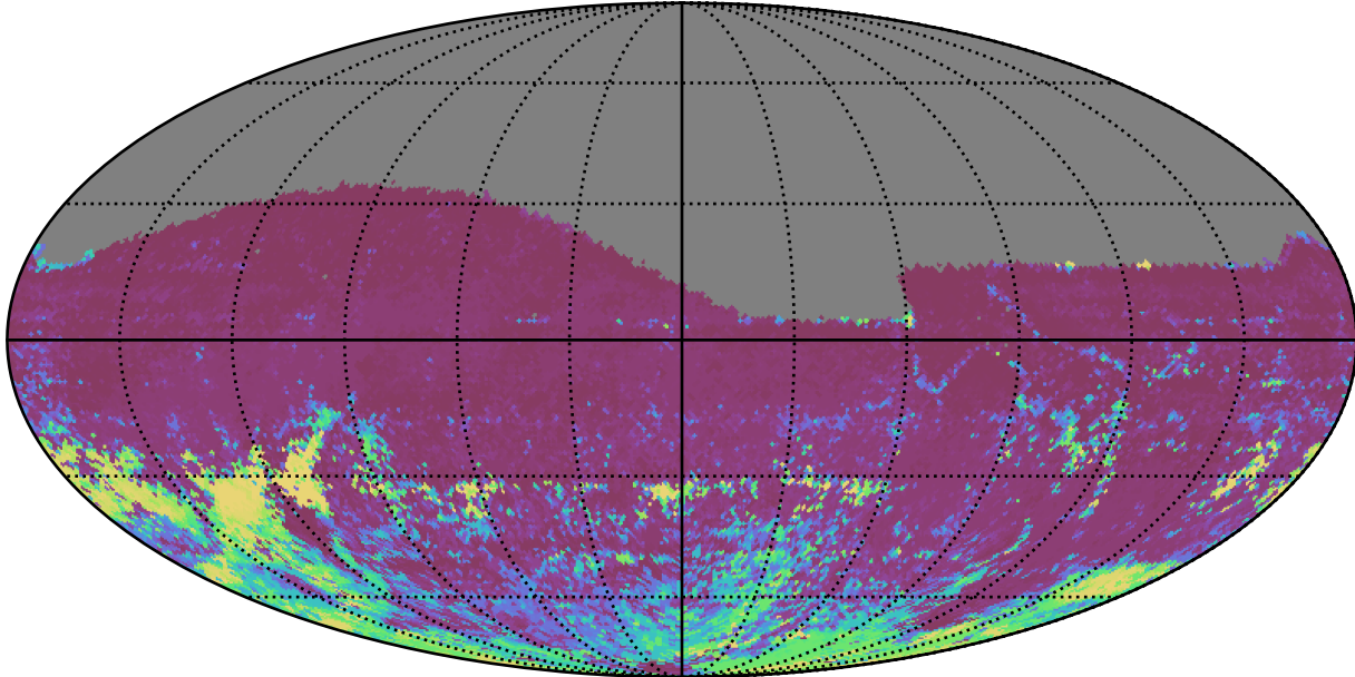
too_elab_r128_d2_gz_v3.4_10yrs All sky r band: 75th Percentile Intranight Timespan
