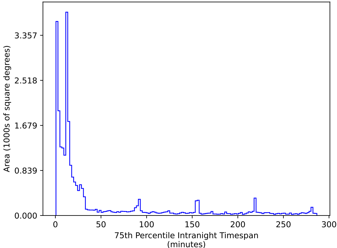
too_elab_r128_d2_gz_v3.4_10yrs All sky r band: 75th Percentile Intranight Timespan
