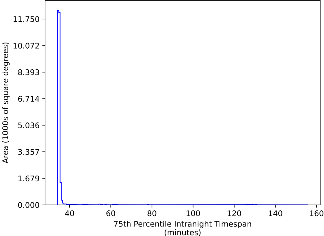
too_elab_r128_d2_gz_v3.4_10yrs All sky iz bands: 75th Percentile Intranight Timespan
