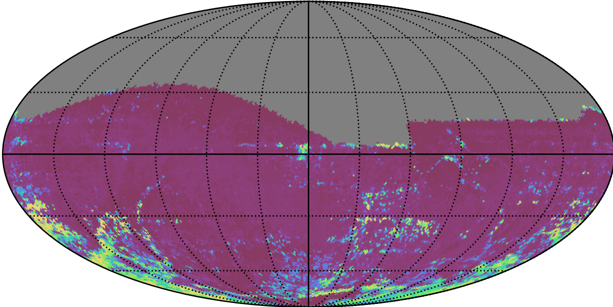
too_elab_r128_d2_gz_v3.4_10yrs All sky i band: 75th Percentile Intranight Timespan
