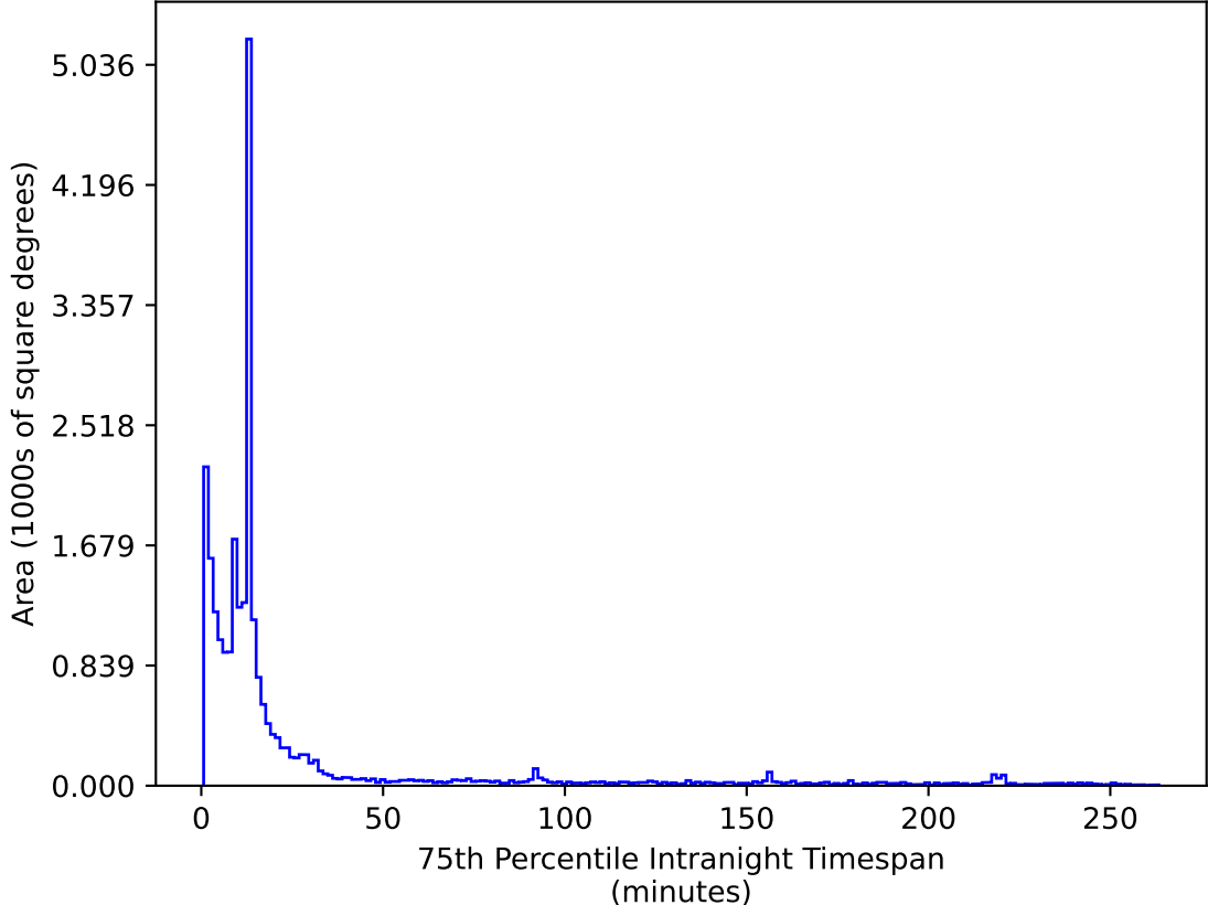
too_elab_r128_d2_gz_v3.4_10yrs All sky i band: 75th Percentile Intranight Timespan
