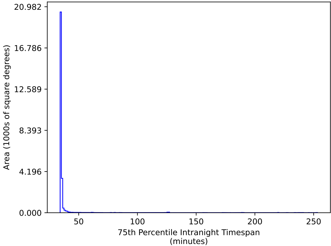
too_elab_r128_d2_gz_v3.4_10yrs All sky gr bands: 75th Percentile Intranight Timespan
