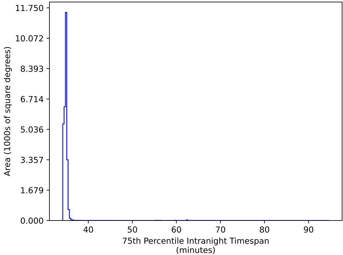
too_elab_r128_d2_gz_v3.4_10yrs All sky all bands: 75th Percentile Intranight Timespan
