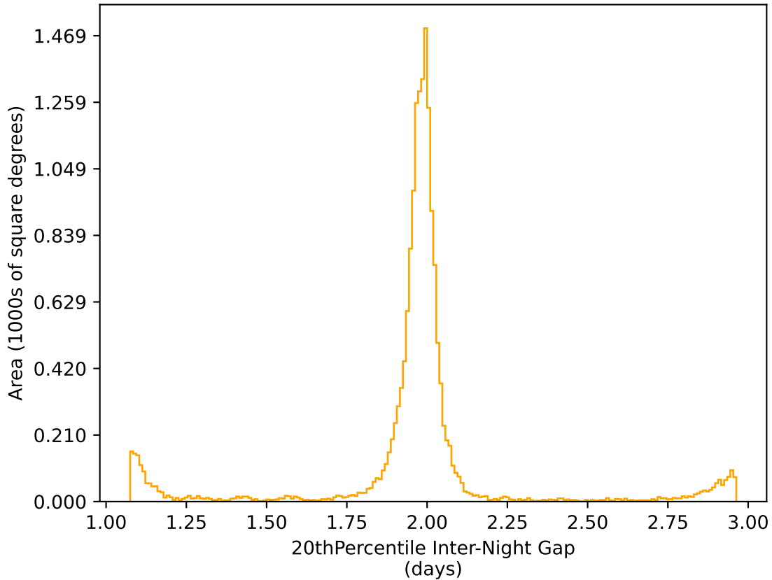
too_elab_r128_d2_gz_v3.4_10yrs WFD r band: 20thPercentile Inter-Night Gap
