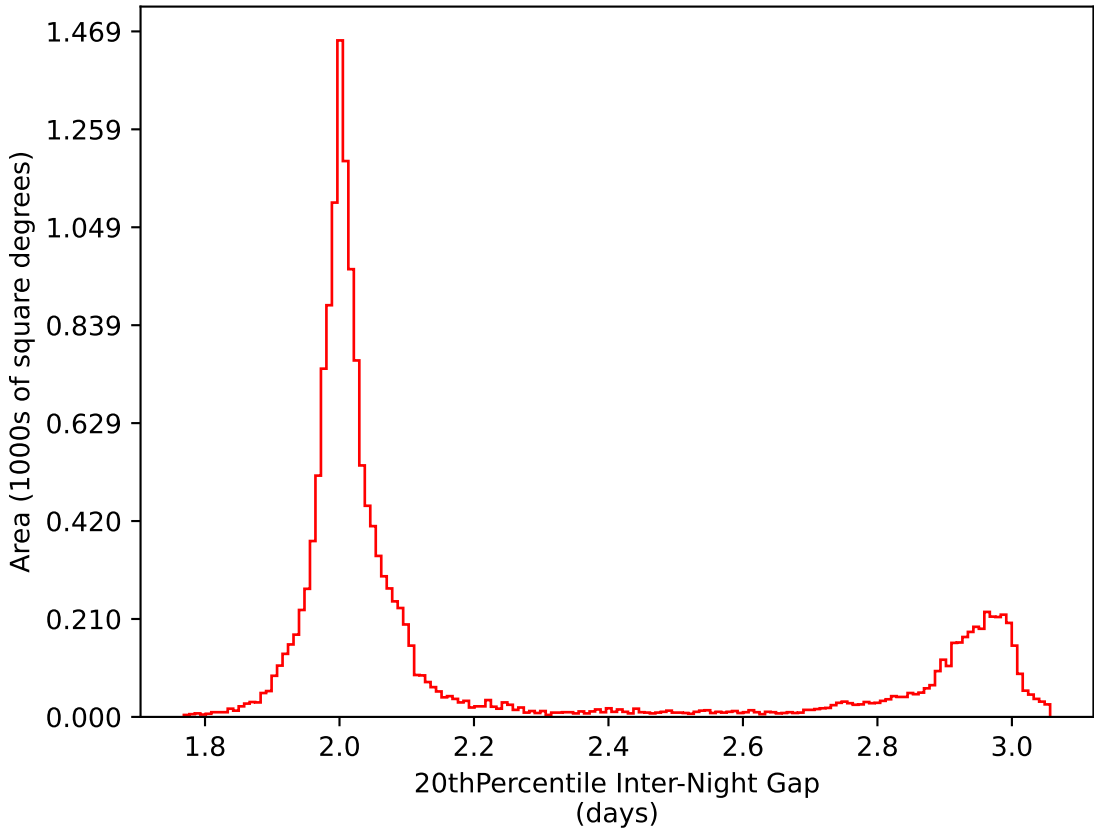
too_elab_r128_d2_gz_v3.4_10yrs WFD i band: 20thPercentile Inter-Night Gap
