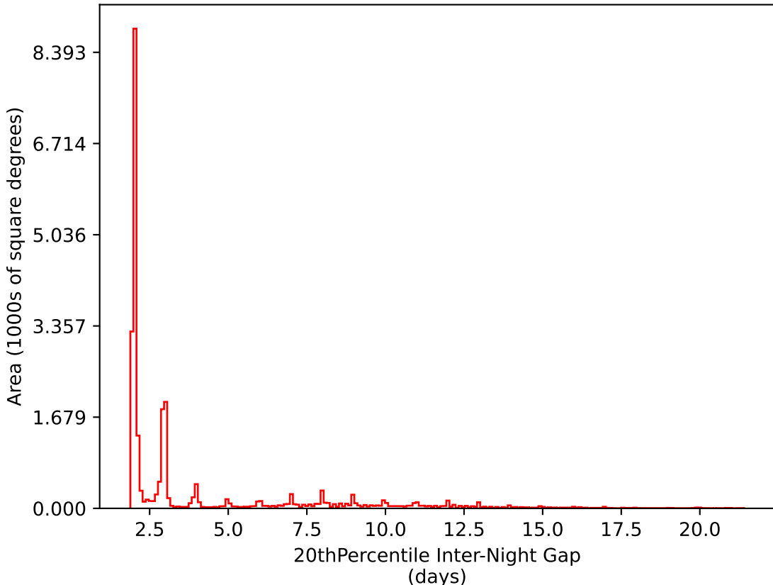
too_elab_r128_d2_gz_v3.4_10yrs All sky i band: 20thPercentile Inter-Night Gap
