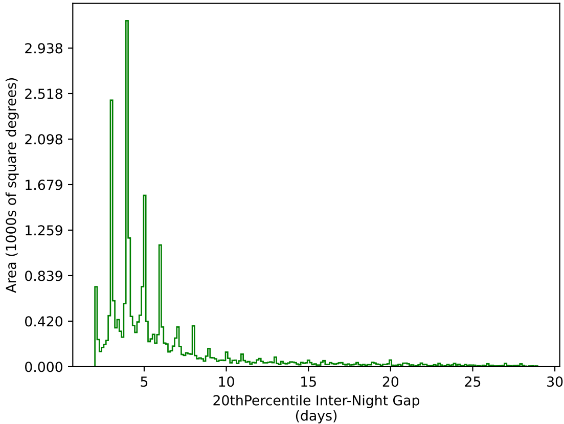
too_elab_r128_d2_gz_v3.4_10yrs All sky g band: 20thPercentile Inter-Night Gap
