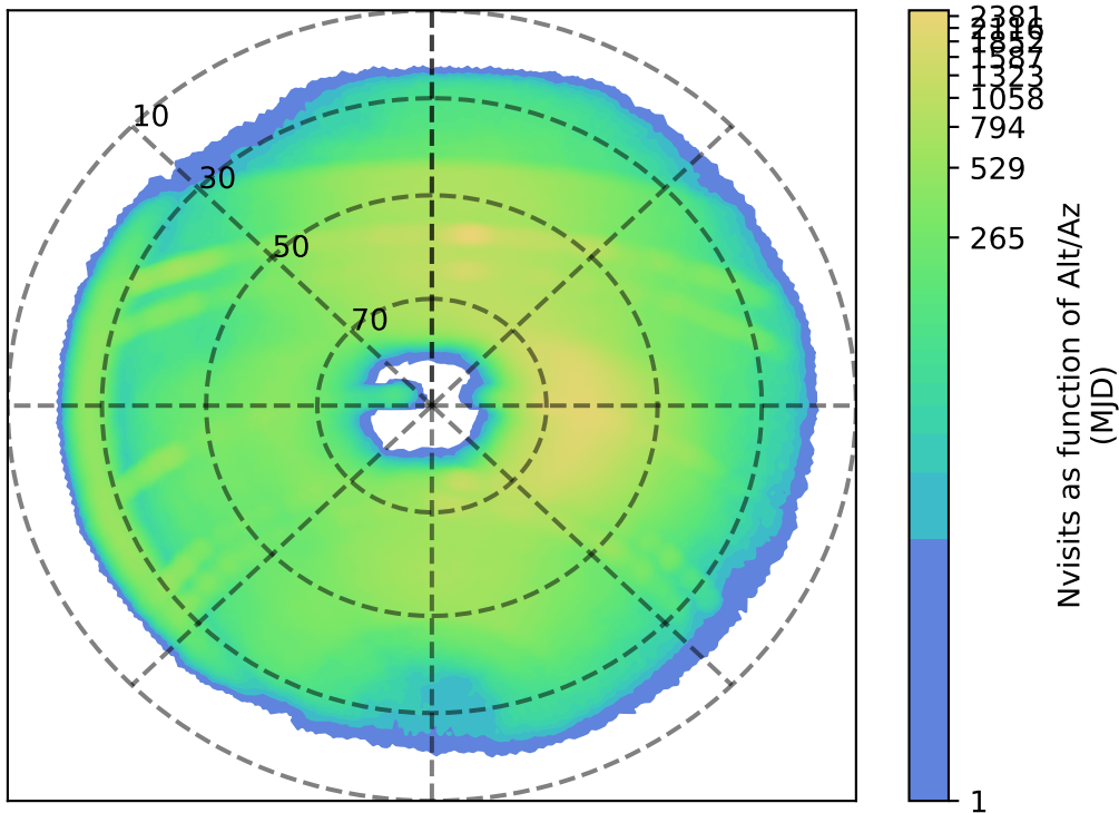
too_elab_r128_d2_gz_v3.4_10yrs r: Nvisits as function of Alt/Az
