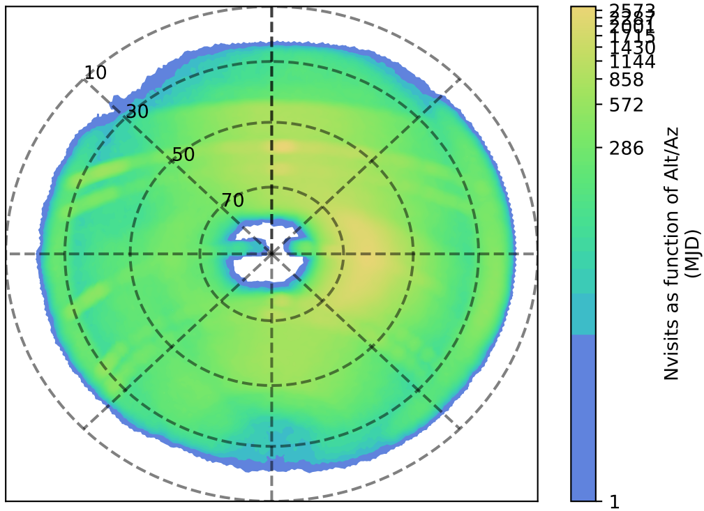
too_elab_r128_d2_gz_v3.4_10yrs i: Nvisits as function of Alt/Az
