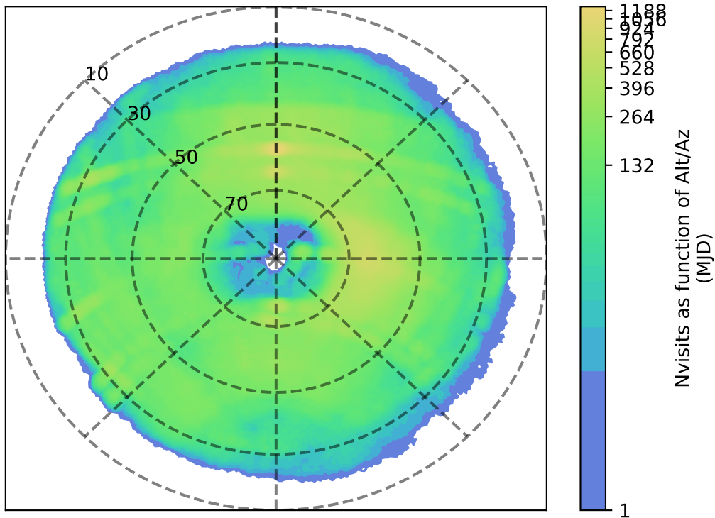
too_elab_r128_d2_gz_v3.4_10yrs g: Nvisits as function of Alt/Az
