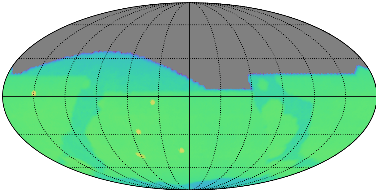
too_elab_r128_d2_gz_v3.4_10yrs : CoaddM5
